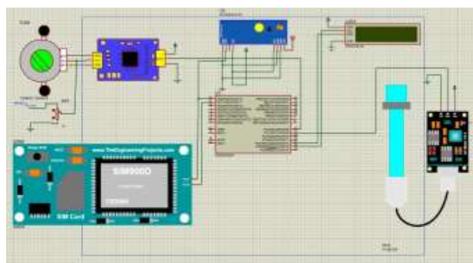
Fig. 3. Water quality system schematic diagram
